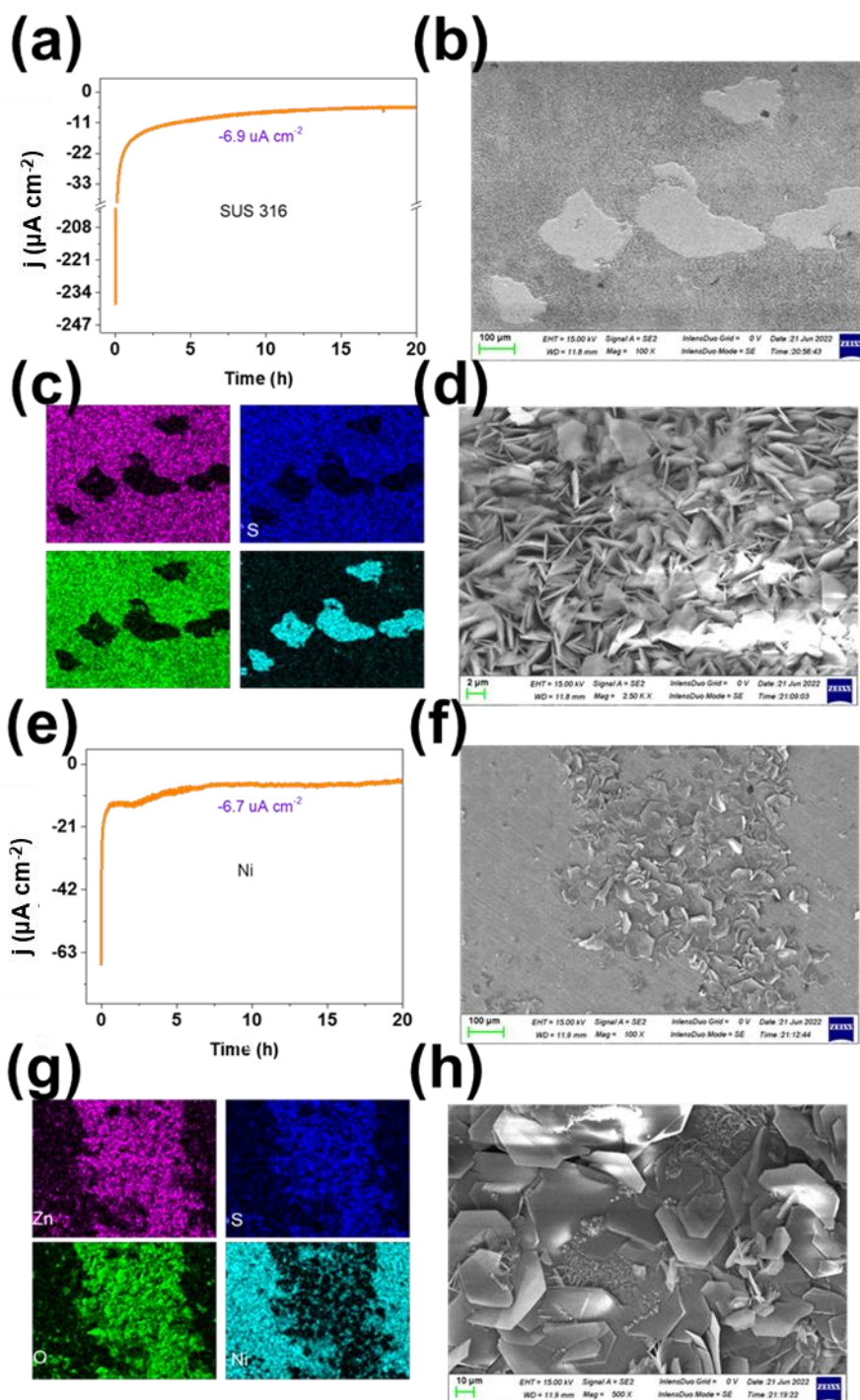
Figure 2.7 Potentiostatic curves of SUS 316 and Ni substrates and its surface component observation. Current density curves of (a) SUS 316 and (e) Ni substrate. The values inside the figures are the stabilized current after the initial period. SEM and elemental mapping of surface components after potentiostatic measurement on (b-d) SUS 316 substrate and (e-h) Ni substrate.
